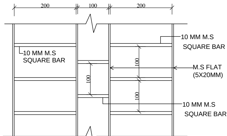
TYPICAL WINDOW AND VENTILATOR GRILL DETAIL
