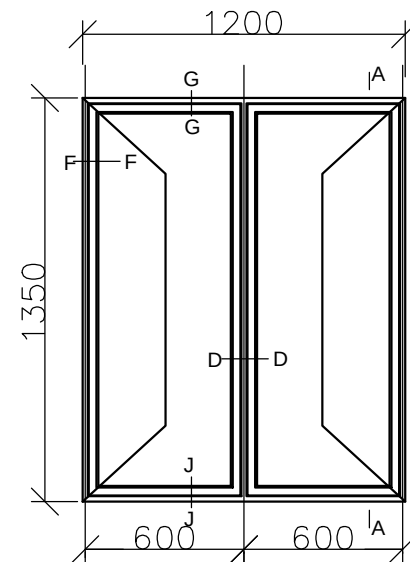
WINDOW TYPE W1V1
