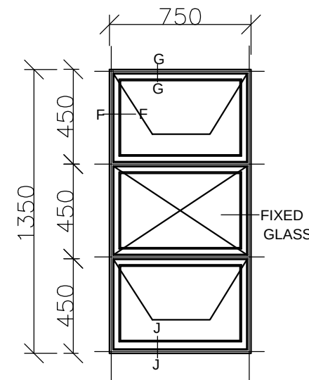
WINDOW TYPE W3V3
