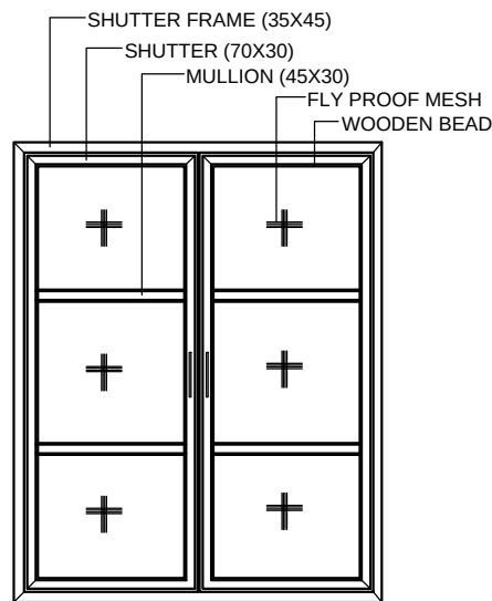
TYPICAL WINDOW AND VENTILATOR FLY PROOF DETAIL
