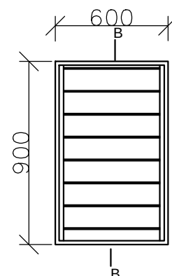
WINDOW TYPE W5 (LOUVERS)
